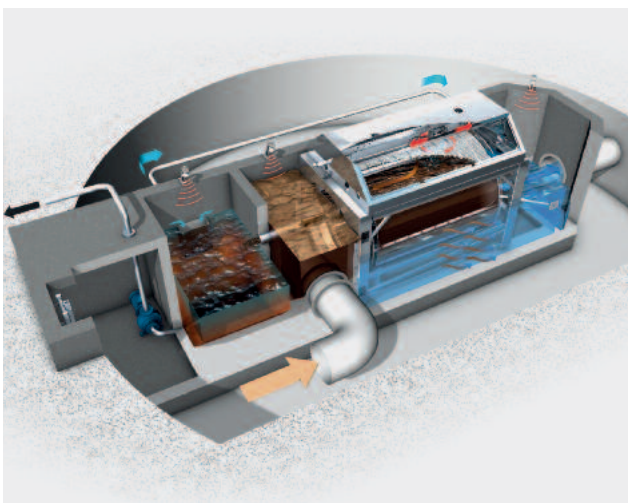
CarbonWin® System: the better primary settlement tank for optimal reduction rates (see separate brochure)
